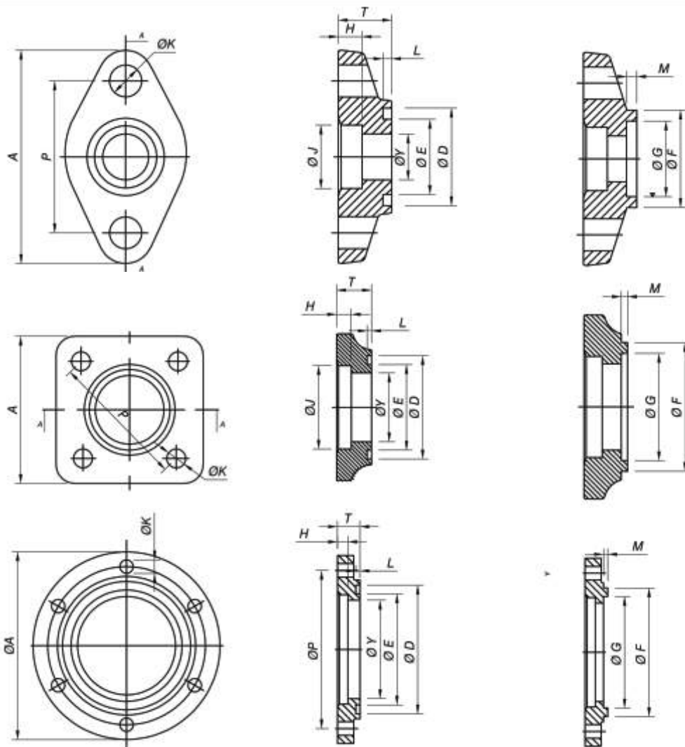
DIMENSION DETAILS OF SOCKET WELD FLANGE
